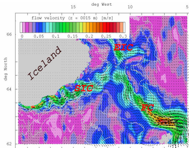
Figure. 1 Simulated 1992-2006 mean current at the depth of 15 m south-east of Iceland and bottom topography (200, 500, 1000 and 1500 m isobaths).
